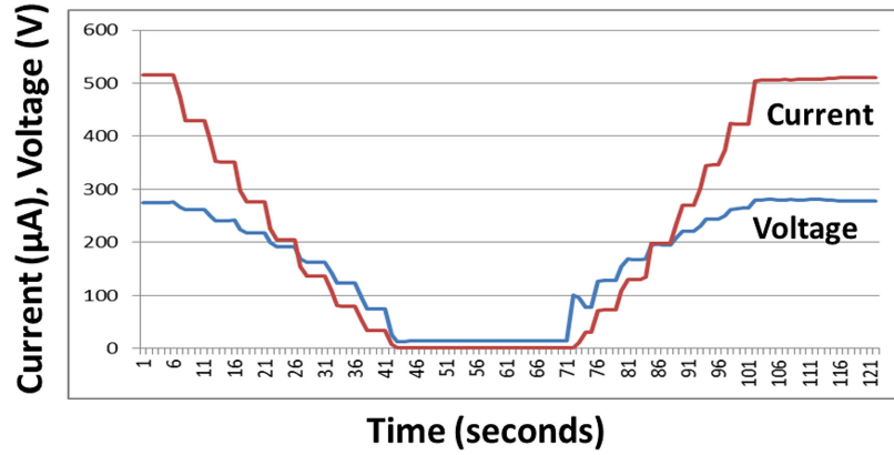
Figure 4. Measured I-V characteristic of a LEC cell tested at -55 °C conducted over a 2 minute time period.
