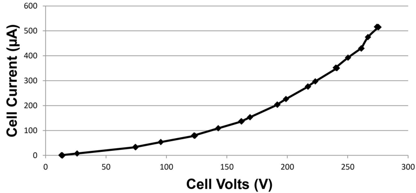
Figure 4. I-V relationship between current and voltage at -55°C.
