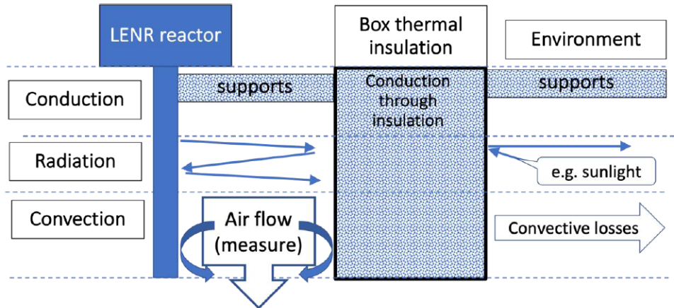
Figure 2. Heat transfer phenomena in AFC.
