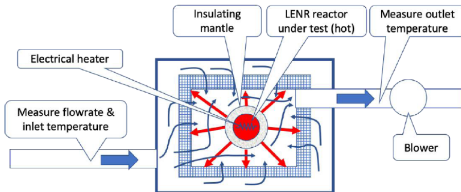
Figure 9. Schematic AFC setup to test a high temperature reactor (with TCS).
