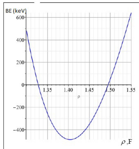
Figure 6. Plot of electron BE for 1.3 F < \rho < 1.55 F .
