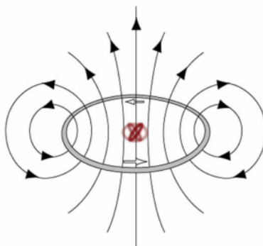
Figure 11. Illustration of the stabilized electron orbit. The gray ring represents the electron's zitterbewegung orbit, the arrows represent magnetic field lines, and the red rings represent the proton's precessing zitterbewegung motion.
