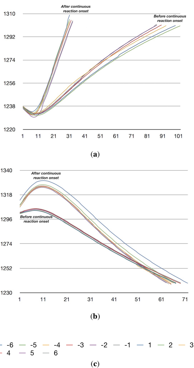
Figure 3. Temperature (°C) vs. time (s) charts during transition from bursty to continuous process with Ni-Cu-Li fuel mixture. (a) heating phases (constant heating power). (b) Cooling phases (zero heating power). The labels (c) indicate cycle no. relative to the starting of continuous reaction.
