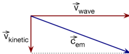
Figure 8. Illustration of the equivalence between instantaneous electron speed vectors in the case of purely wave-like zitterbewegung rotation (blue) and the particle-like case of composition between mechanical plus wave-like zitterbewegung rotations (red).
