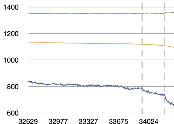
Figure 5. Temperature and heating power evolution of a reactor containing Li–Ni–Al fuel composition. The green curve shows the temperature (°C) at the fuel container, the yellow curve shows the temperature (°C) at the edge of reactor, and the blue curve shows the applied heating power (W). The horizontal axis indicates the elapsed time (s).
