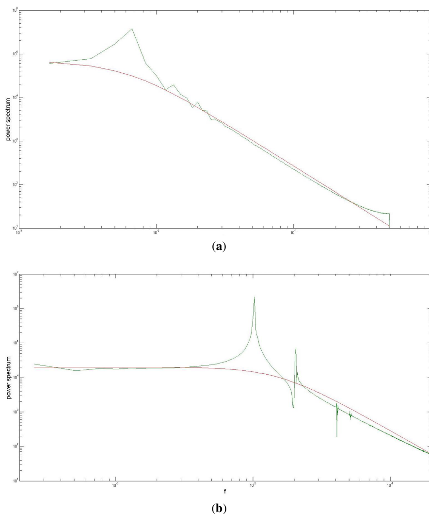
Figure 4. Autocorrelation frequency spectrum during the continuous reaction process with Ni–Cu–Li fuel mixture. (a) The spectrum prior to the continuous reaction and (b) the spectrum during the continuous reaction.
