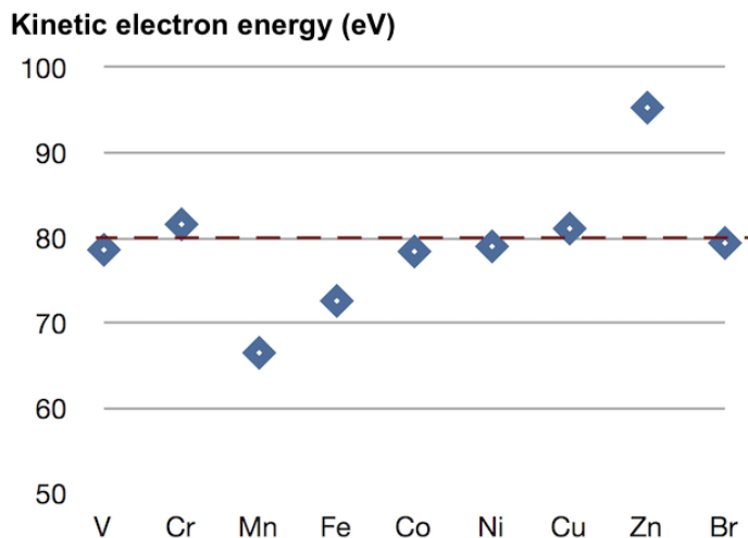
Figure 12. Display of electron energies which are closest to the 80 eV level, shown for elements around Ni.
