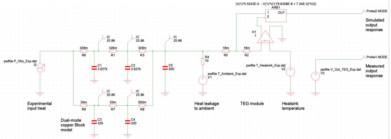
Figure 22. Second pass dual mode model.
