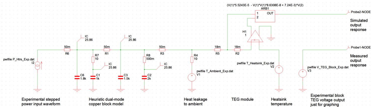
Figure 23. Third pass heuristically derived model.
