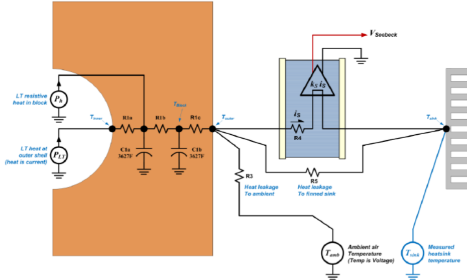
Figure 12. Reduced circuit model.
