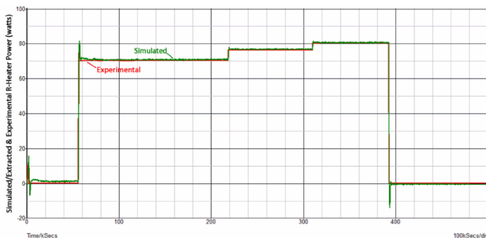
Figure 30. Simulation extracted null LT heater waveform.
