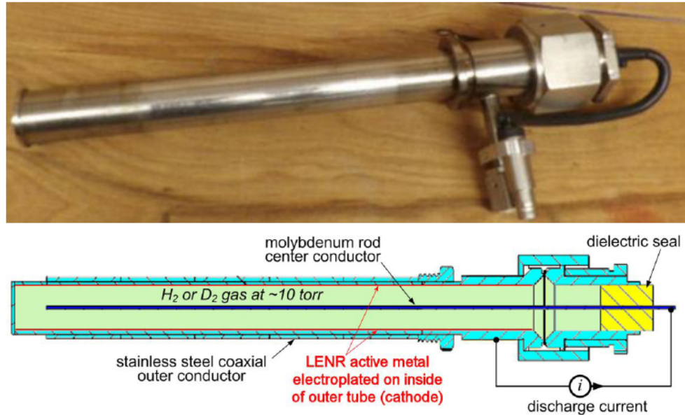
Figure 6. Gas discharge “LENR Tube” (LT).
