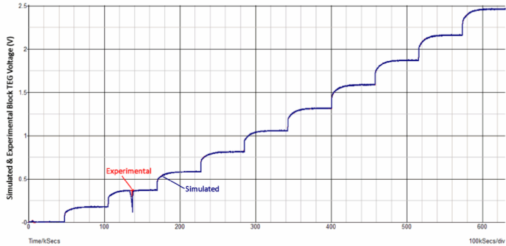
Figure 24. Stair-step response of third pass model.
