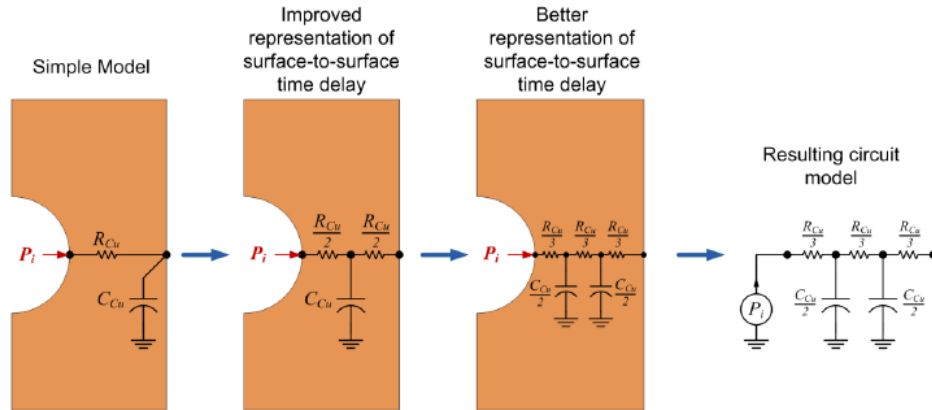
Figure 9. Dynamic thermal model for copper block.
