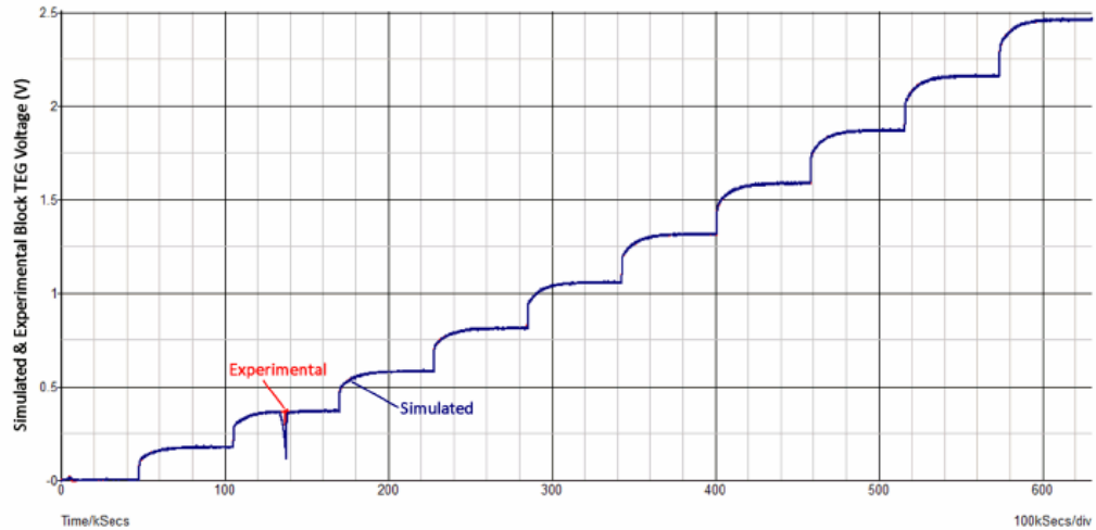
Figure 27. Fourth pass model block TEG response.
