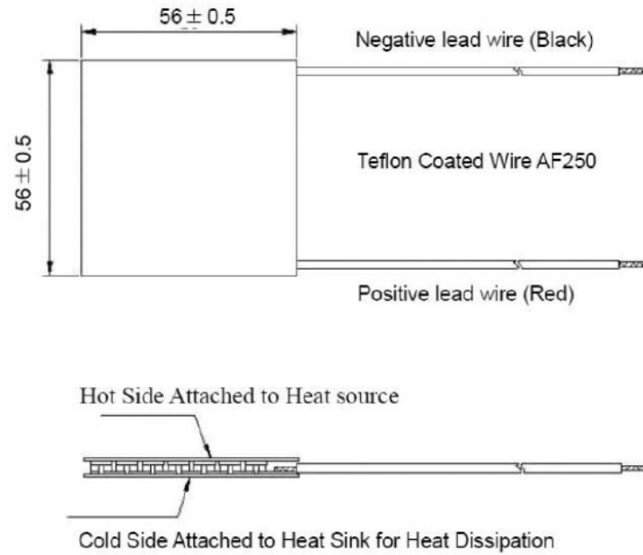
Figure 4. TECTEG TEG1-12611-6.0 TEG module drawing.
