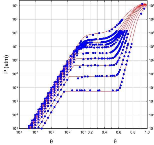
Figure 4. Model isotherms ( red lines ) and input isotherm points ( blue circles ) for \text{PdH}_x . The isotherms from lowest to highest correspond to temperatures of for (from lowest to highest curves) T = 293, 343, 393, 433, 473, 516, 543, 573, 613 , and 710 K.
