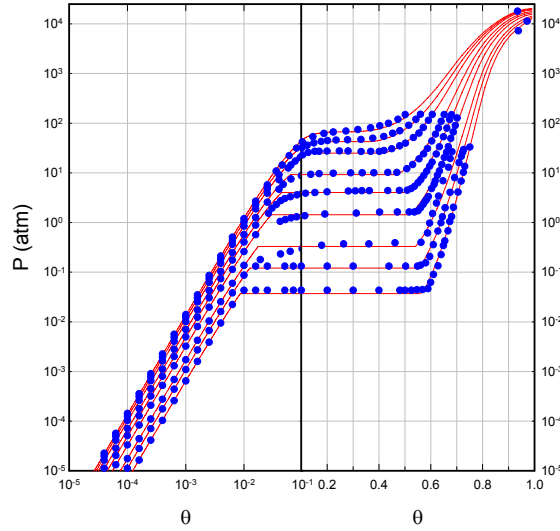
Figure 2. Model isotherms (red lines) and input isotherm points (blue circles) for \text{PdD}_x .
