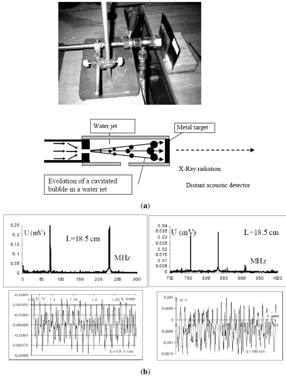
Figure 1. General view and scheme of experimental setup and the view of signals (frequency spectrum and structure of time dependence) registered in air by broadband acoustic piezoceramic detector at distances L = 18.5 cm and L = 198 cm from the outer surface of the tungsten target.
