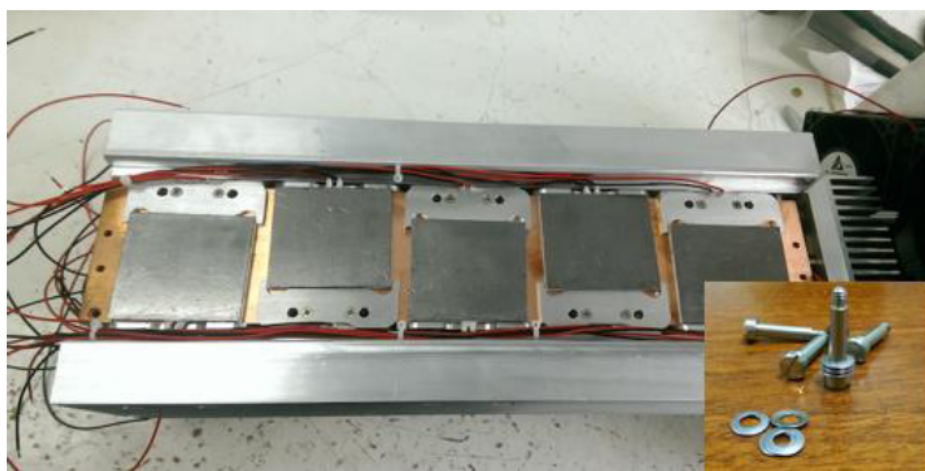
Figure 4. Figure shows how the thermoelectric devices are attached to the copper block using Bellville washers, shown in the inset. The Bellville washers provide a constant force to the heat fins as they press against the thermoelectric devices.
