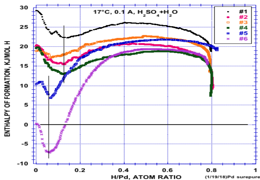
Figure 8. Total enthalpy of formation as a function of H/Pd for the various loading–deloading cycles that resulted in the thickness change shown in Fig. 5. The values apply to the reaction \text{Pd} + (x/2)\text{H}_2 = \text{PdH}_x .
