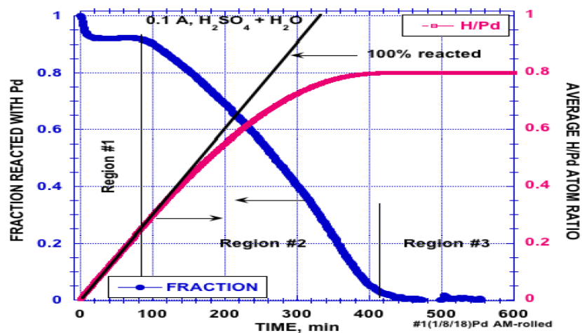
Figure 3. Example of fraction of H reacting as a function of time and the resulting average H/Pd ratio. Initially, nearly every H released from H_2O reacts with Pd ( Region #1 ). Upon reaching the H/Pd ratio limit, the net amount of H reacting with the PdH is zero ( Region #3 ) because H_2 leaves the sample as fast as it is applied by electrolytic action. Because every sample shows different behavior, the H/Pd ratio can not be obtained using the theoretical loading behavior as has been done by some researchers in the past.
