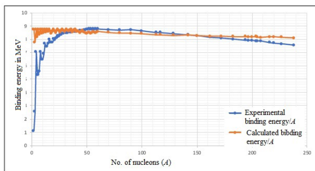
Figure 2. Plots of the experimental nuclear binding energy per nucleon (blue) and the simple calculated binding energy (orange), taking into consideration the quantum rules of hard-core repulsion and zero electric dipole moment. This is based on the number of possible quantum-allowed up-to-down quark pairs and a fixed binding energy per bonded pair.
