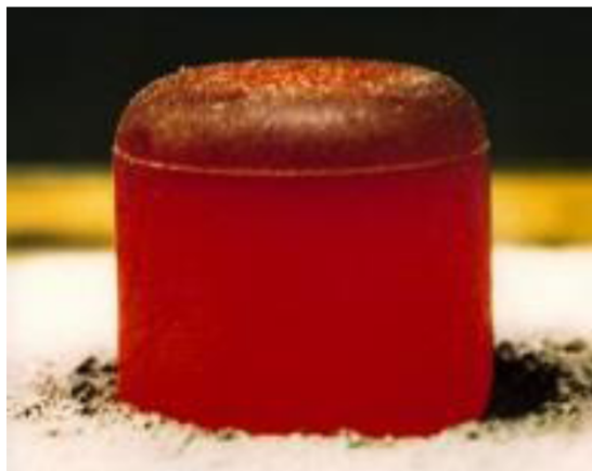
Figure 1. A spontaneously warm pellet of pure ^{238}\text{Pu} . In the picture, the metallic pellet is red hot after its insulation (to contain the heat) was removed. As with LANR, this so-called “free energy” is actually from nuclear de-excitations.
