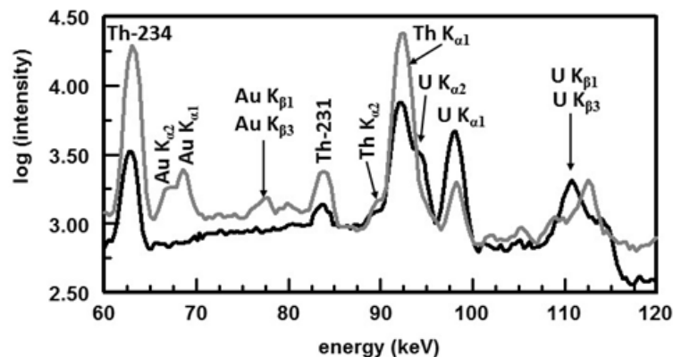
Figure 6. Gamma ray spectra, between 60 and 120 keV, of the native uranium wire ( black ) and the Au/U/Pd composite cathode ( gray ) at the end of the experiment. Peak assignments are shown [17].
