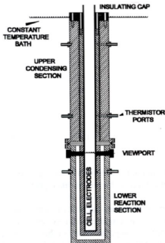
Figure 1. Schematic of the ICARUS-9 calorimeter.
