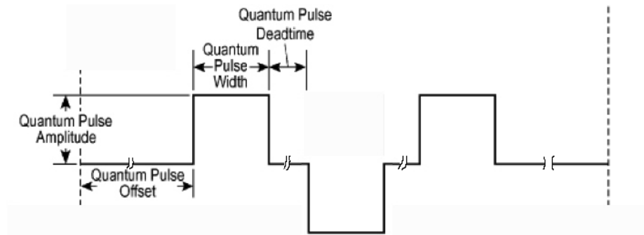
Figure 2. Example of Brillouin's "Q-Pulse".
