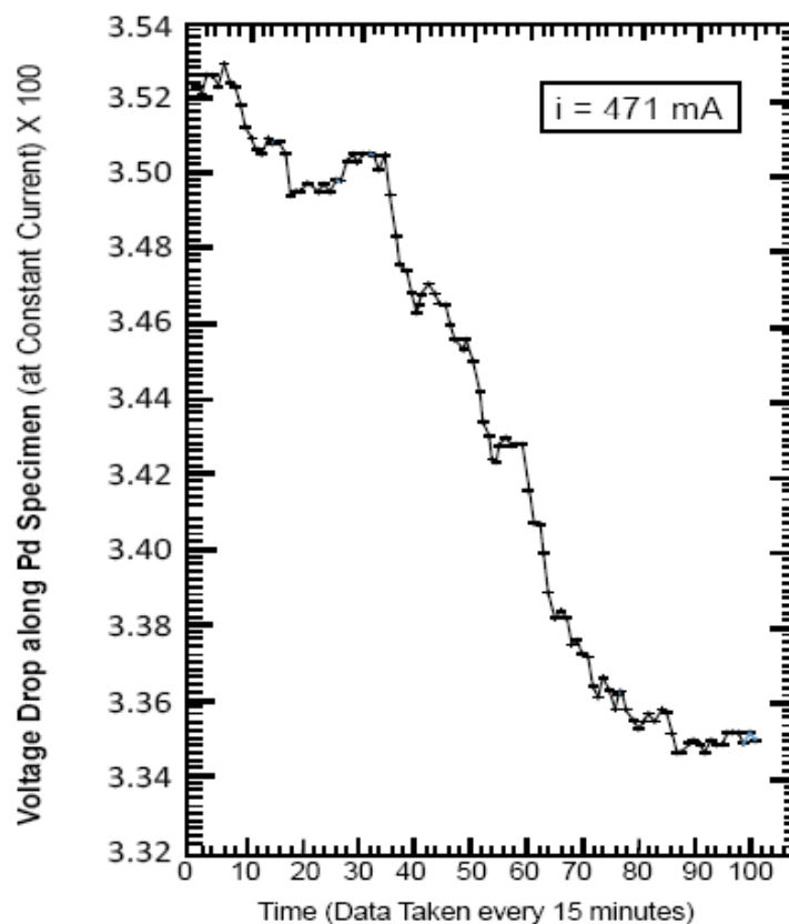
Figure 23. Left cell (Pd/Pt) in D_2O exhibiting excess power (+). The resistivity of the PdD had gone over the hump in resistance (near D/Pd = 0.74 ) at the beginning of the run assuring specimen is in the range above an average D/Pd = 0.93 for the events featured here. The drop in voltage along specimen is from a change in its resistivity since electromigration current is constant and the temperature of the cell is increasing.
