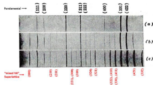
Figure 37. Powder XRD pattern (reflection line intensity recorded on film) of the development of order in an FCC Au–Cu alloy: (a) disordered (fundamental reflections), (b) partially ordered, and (c) highly ordered \text{AuCu}_3 with Superlattice reflections, adapted from [92].
