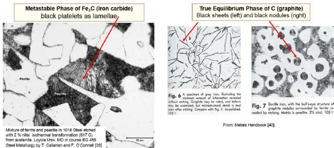
Figure 2. Micro-constituents for the diagrams in Fig. 1: those on the left (from [39]) are for the metastable Fe– \text{Fe}_3\text{C} phase diagram, those on the right (from [40]) are for the true equilibrium Fe–C diagram, showing that both types of diagrams are useful for steel and cast iron.
