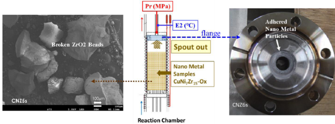
Figure 6. Examples of broken ZrO 2 beads and adhered nano-material on the upper flange after excess heat generation.
