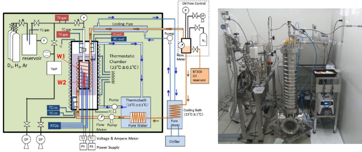
Figure 2. Experimental set-up.
