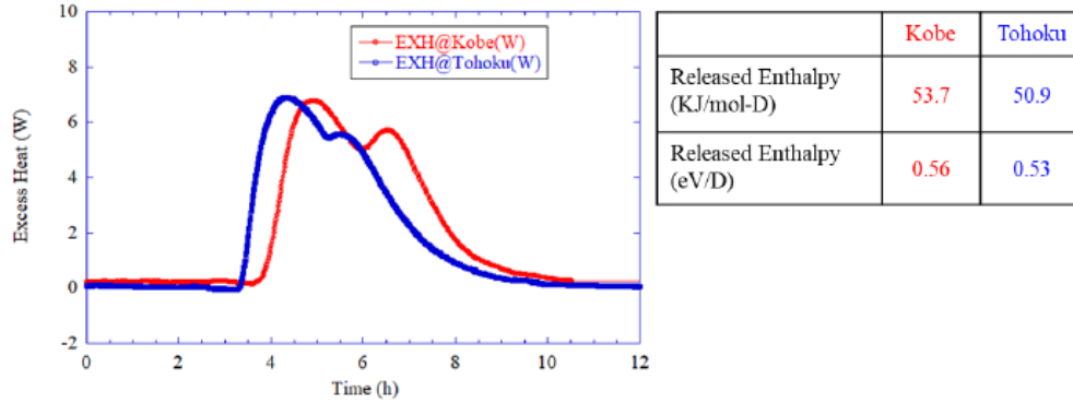
Figure 8. Comparison of released heat power between Kobe and Tohoku at room temperature..
