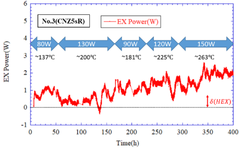
Figure 3. An example of excess heat generation; CNZ5sR with H_2 .
