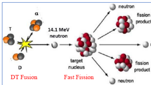
Figure 10. DT Fusion-fast-fission reaction.
