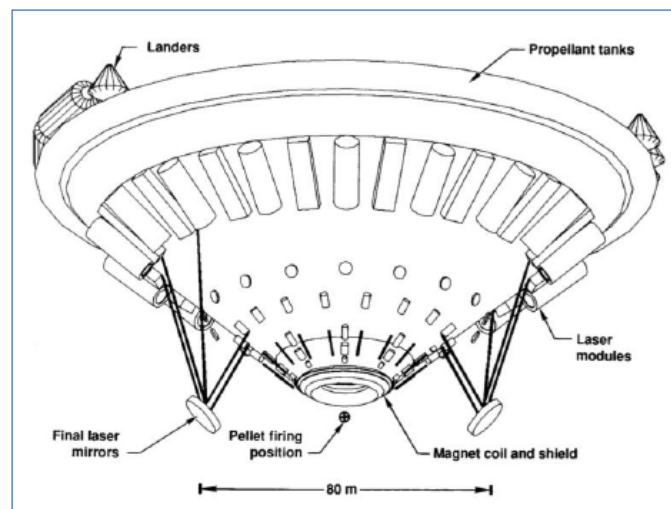
Figure 4. Laser fusion propulsion.
