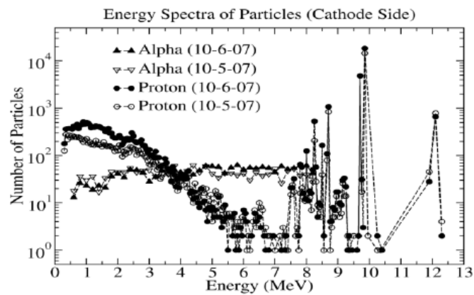
Figure 6. Pd/D Charged particle spectra 1–13 MeV [17].
