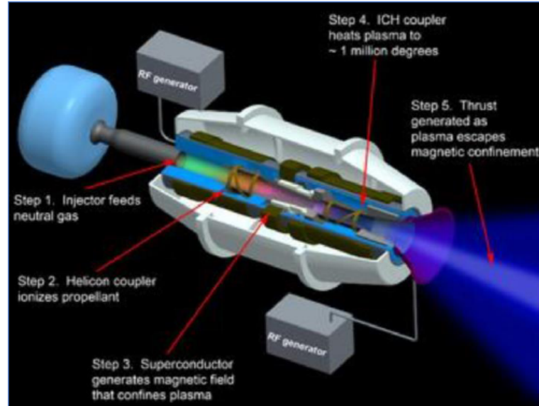
Figure 5. VASIMR propulsion.
