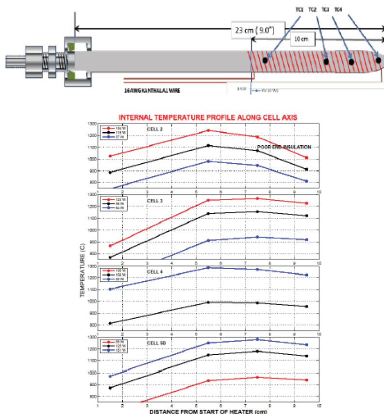
Figure 2. Temperature variation along the axis of cells
