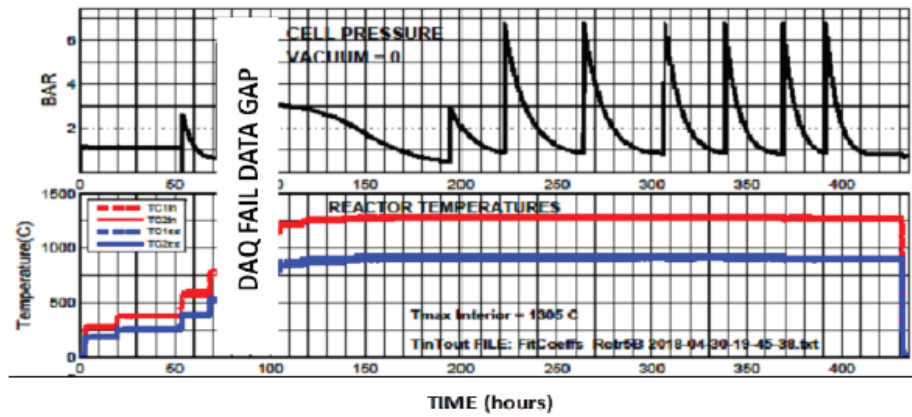
Figure 9. Data run interrupted by ICCF-21 conference.
