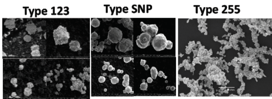
Figure 7. Electron micrographs of three types of Vale nickel powder.
