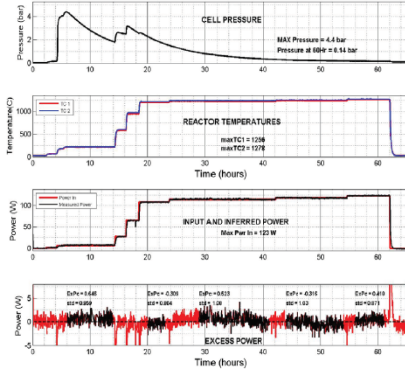
Figure 8. One-time pressure profile of a mixture of nickel powder and \text{LiAlH}_4 .
