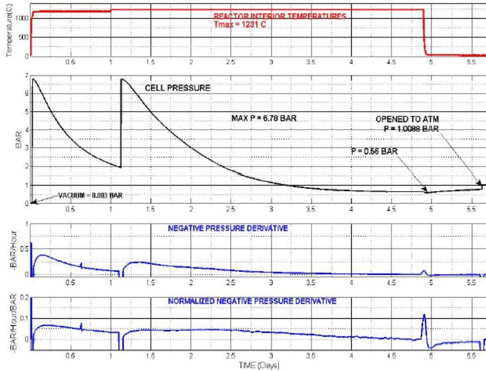
Figure 10. Pressurization of an empty cell.
