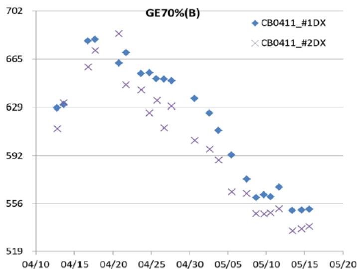
Figure 3. The change of \gamma -ray counting rate ( s^{-1} ) from ^{137}\text{Cs} over time (month/day).
