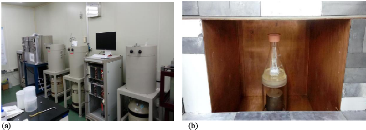
Figure 2. The experimental setup equipped with high-purity Ge detector (a), and the sample flask above the detector (b).
