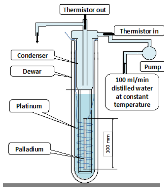
Figure 1. Schematic of the electrolytic cell.
