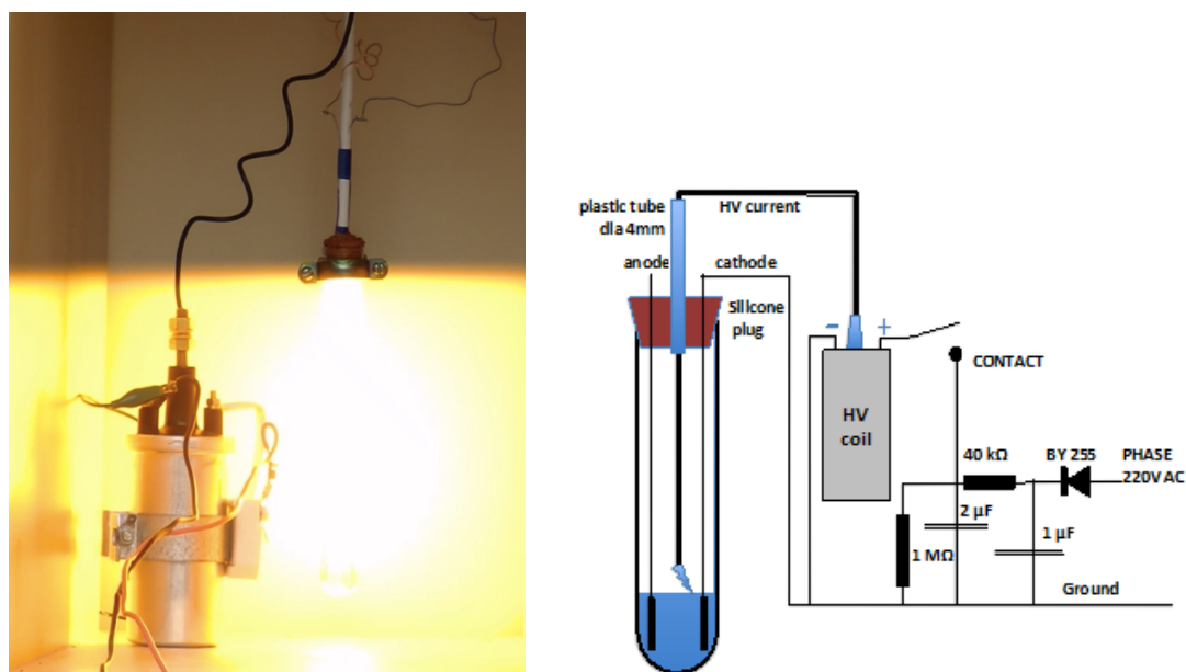
Figure 14. Explosion ignited by a high voltage spark.
