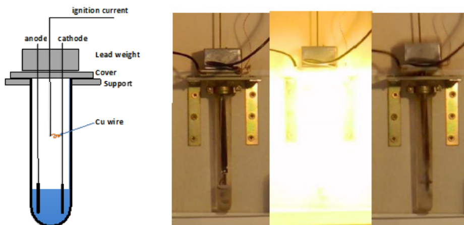
Figure 15. Ignition by an exploded wire. The tube is plugged by a lead weight, free to lift under the influence of the gas pressure. Pictures are taken at 33 ms intervals. The maximum altitude reached by the weight makes it possible to obtain a rough estimate of the gas pressure.
