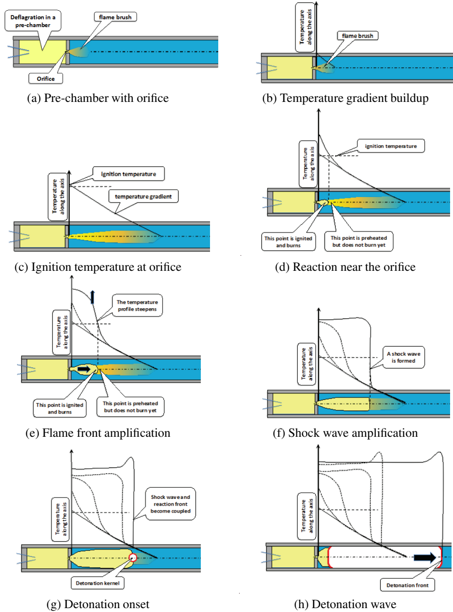
Figure 12. The SWACER detonation mechanism.
