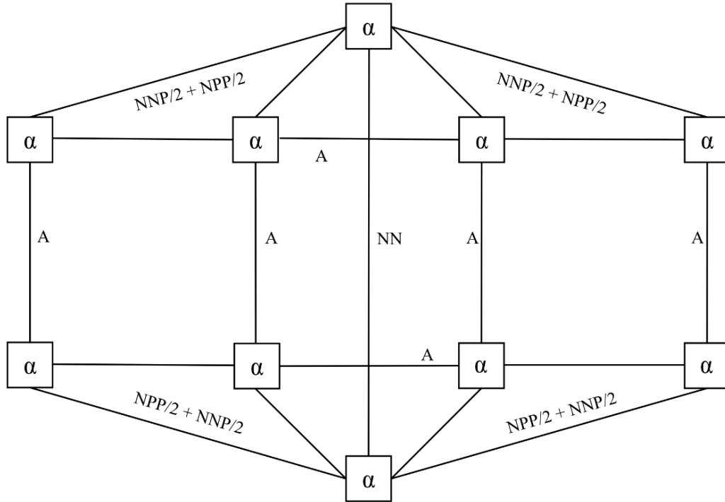
Figure 3. Distribution of E_B \text{Ca}^{40} between \alpha particles.
