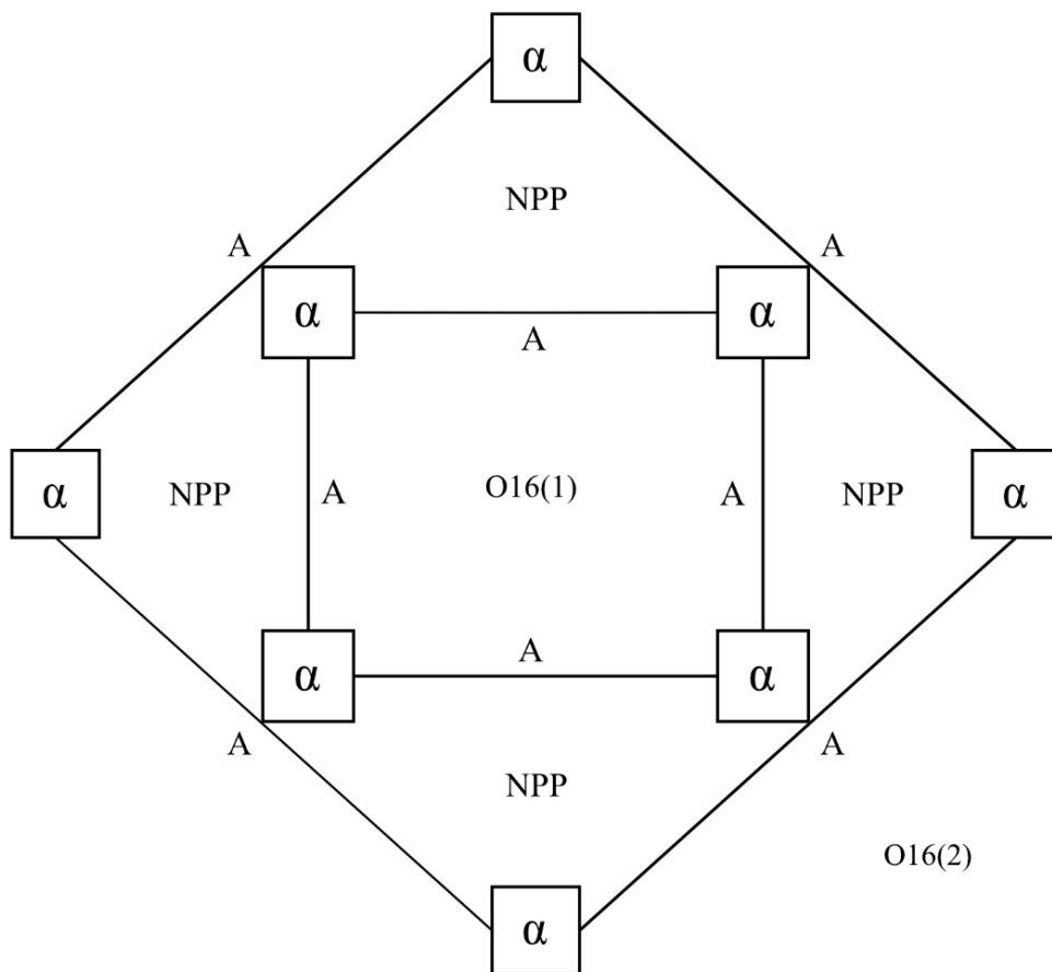
Figure 2. Tentative transmutation process. Basis: Two structures of O 16 with each 4A bonds.
