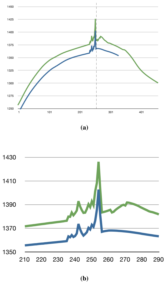
Figure 23. Temperature evolution measured by the first ( blue ) and second ( green ) thermocouple. The dashed line indicates loss of heating due to wire breaking.
