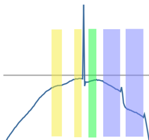
Figure 5. Temperature curve around the reaction event, the shading highlights the reaction related events.
