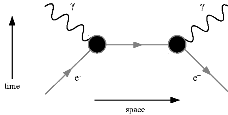
Figure 4. Feynman’s diagram of positron–electron annihilation.
