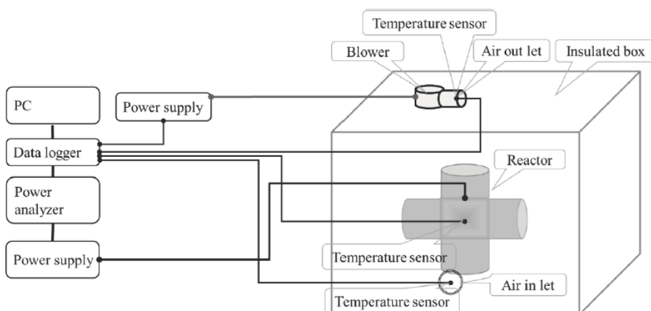
Figure 13. Schematic of measurement system.
