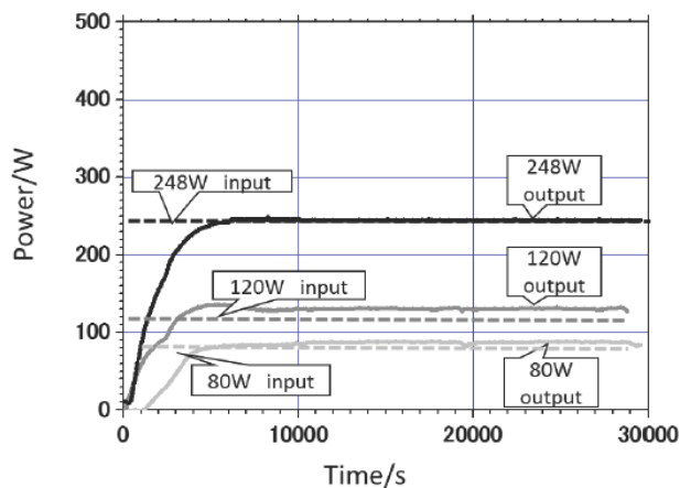
Figure 27. Change in output for calibration reactor.
