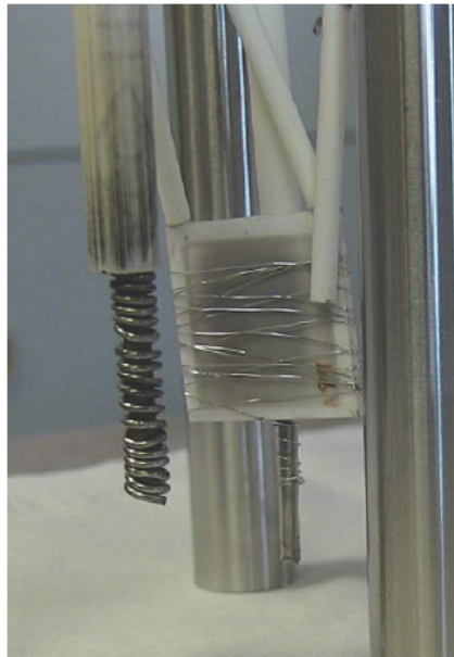
Figure 5. View of the electrode and heater in the reactor.
