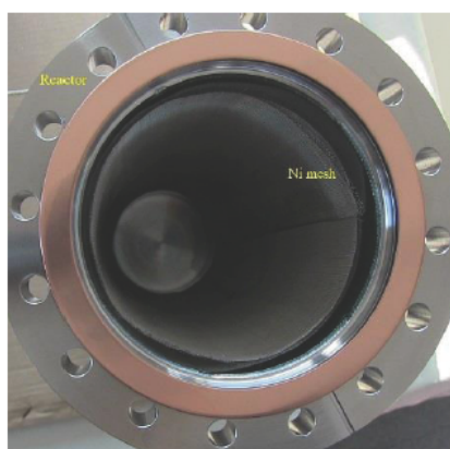
Figure 3. View of Ni mesh in the reactor.
