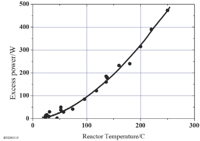
Figure 30. Relationship between excess power and reactor temperature.
