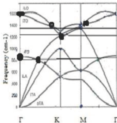
Figure 8. Phonon dispersion curves of graphene by Lazzeri et al. [109]. *G peak at 1580\text{ cm}^{-1} corresponds to double degenerance in-plane phonon mode on \Gamma point (stationary vibration mode within hexagonal Csp 2 –Csp 2 cyclic ring). *The so-called D-disorder peak at \sim 1350\text{ cm}^{-1} corresponds to a double degenerance in-plane phonon mode on near K point (Coupled Double Resonance scattering on a symmetric A-edge Csp 2 –Csp 2 bond (external edge of graphene sheet or intern edge of voids in graphene). *The so-called 2D peak at \sim 2700\text{ cm}^{-1} corresponds to addition of D-disorder phonon (2K mode on A-edge), and in the bulk to 2 K and 2 M phonon modes Raman active (single M phonon mode at \sim 1350\text{ cm}^{-1} is not Raman active).
