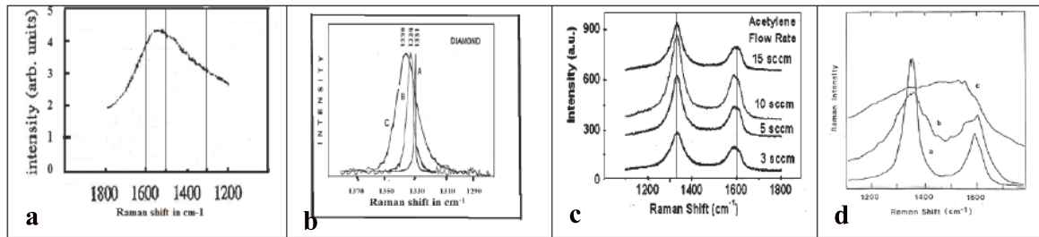
Figure 7. Raman spectra of (a) pseudo-amorphous graphite with few sp 3 and amorphous graphite (GAC) (ion irradiated glassy carbon by Prawer et al. [112] \sim 15 cm -1 stress upshift sp 3 Diamond band and D-disorder (GeA cluster edge \sim 1350/1360 cm -1 . Max intensity GD band 1560 cm -1 Csp 2 –Csp 3 . Weak G-band \sim 1600 cm -1 (sp 2 clusters destroyed by irradiation). Similar to non-stressed amorphous graphite 100% sp 2 (Rouzaud [102]), (b) crystalline/amorphous diamond (D diamond by Huang et al. [111]. Results showing existence of amorphous diamond (symmetric band \sim 1330 cm -1 . Same frequency than ordered diamond peak. No G peak/band. No sp 2 cluster edge GeA band \sim 1350 cm -1 \Rightarrow (no so-called D-disorder at 1350 cm -1 ). No Csp 3 –Csp 2 , no Csp 2 –Csp 3 ), (c) carbon nanofiber (CNF) by Lin et al. [69] G+ 1580 cm -1 , G - (CNT intern walls 1560 cm -1 ), main peak for H6 (hexagonal diamond 1325 cm -1 (sp 2 transformed in sp 3 on outer CNT wall during growth process (plasma). No Csp 3 –Csp 2 band (reduced amount only on interface between inner and outer part of CNW)), and (d) modified glassy carbon (Raman spectra glassy carbon N + irradiated by Iwaki et al. [86] \sim 40 cm -1 stress upshift G \sim 1610 cm -1 , GeA \sim 1390 cm -1 . Amorph. Diamond \sim 1370 cm -1 , sp 3 –sp 2 \sim 1510 cm -1 . Tensile stress downshift ( \sim 30 cm -1 with N 2 exodiffusion). Similar to ta-C).
