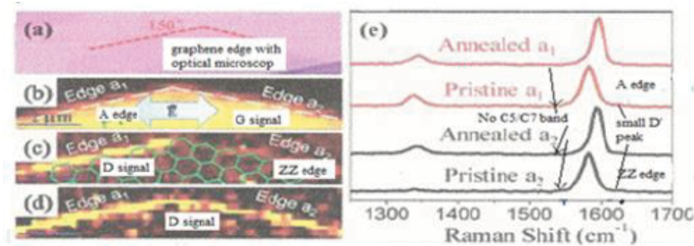
Figure 9. Micro Raman experimental results showing graphene ZZ edge transformation into A-edge with annealing at \sim 300^\circ\text{C} adapted from Xu et al. [119]. No C5/C7 band at \sim 1490/1530\text{ cm}^{-1} . Tensile stress downshift \sim 15\text{ cm}^{-1} on pristine material. The so-called D-disorder peak at 1350\text{ cm}^{-1} localized on external A-edge. D indicates spots in the bulk corresponding to internal A-edge of voids. D' peak (corresponding to edge dangling Csp 2 –Csp 2 ) is reduced with annealing at \sim 300^\circ\text{C} .
