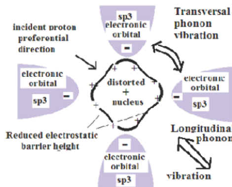
Figure 13. Scheme of electrostatic nuclear barrier distortion with 109° open space sp 3 orbital.
