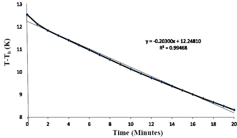
Figure 4. Initial cell cooling for the first 20 min.
