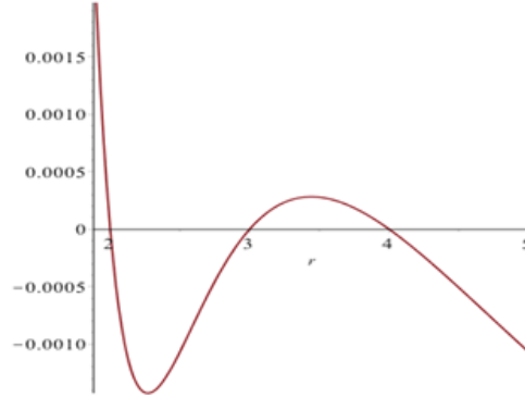
Figure 1. V(r) for r \leq 5 .
