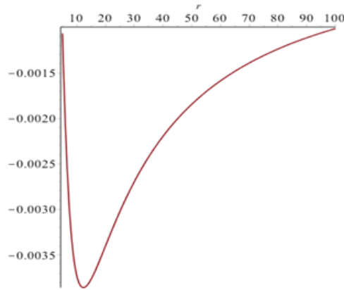
Figure 2. V(r) for 0 \leq r \leq 100 .
