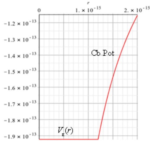
Figure 7. \text{Pot}_\varepsilon(r) with \varepsilon = 10^{-5} .
