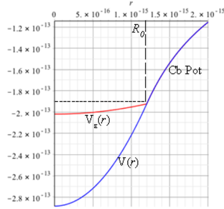
Figure 6. \text{Pot}(r) and \text{Pot}_\varepsilon(r) with \varepsilon = 10^{-1} .
