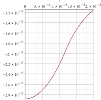
Figure 4. Pot( r ) on interval [0F, 2F] .
