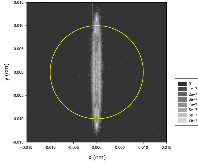
Figure 8. Beam partially focused in x and defocused in y at image plane located at Z = 25 cm in the case of a dipole density of 10^9 \text{ cm}^{-2} . Marked in yellow is a circle of radius 100 \mu\text{m} .
