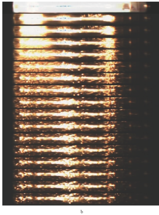
(b) Set of frames from high-speed camera
