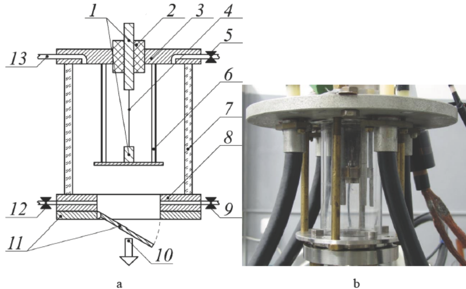
Figure 2. Blast chamber: (a) 1 – mounting electrodes; 2 – insulator; 3 – top flange; 4 – wire; 5 – leak valve for the inlet of argon; 6 – current-return pathway; 7 – chamber wall; 8 – lower flange; 9 – valve for MS-200; 10 vacuum pumping; 11 – gate; 12 – MS-40 valves; 13 – hole for pressure lamp connection. (b) photo of the quartz blast chamber.
