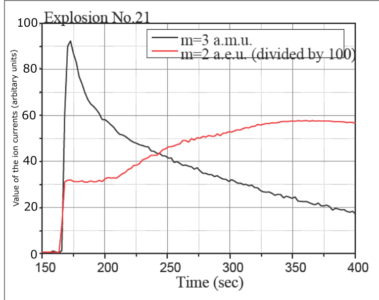
Figure 8. The time dependence of peaks m = 2 a.m.u. and m = 3 a.m.u.
