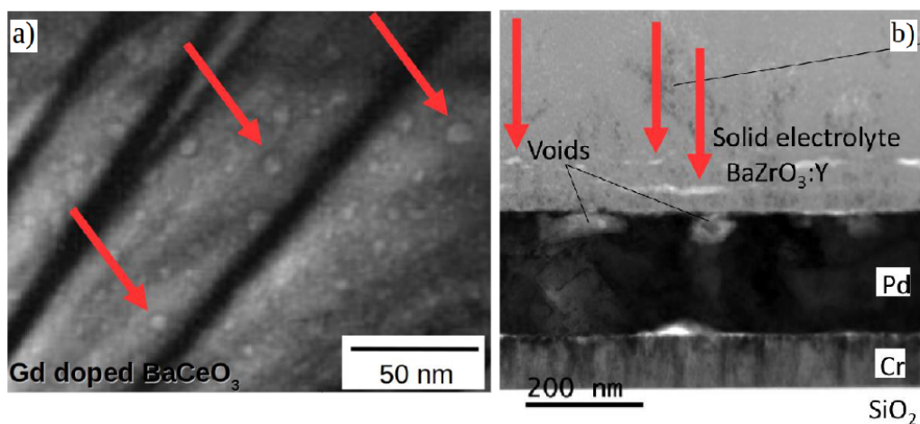
Figure 10. TEM images of nanometric cavities in polycrystalline proton conductors. Red arrows highlight some nanometric cavities. (a) Plane view in Gd-doped BaCeO 3 used below 770 K. From [41]. (b) Cross-section side view in Y-doped BaZrO 3 used at 590 K. From [42].
