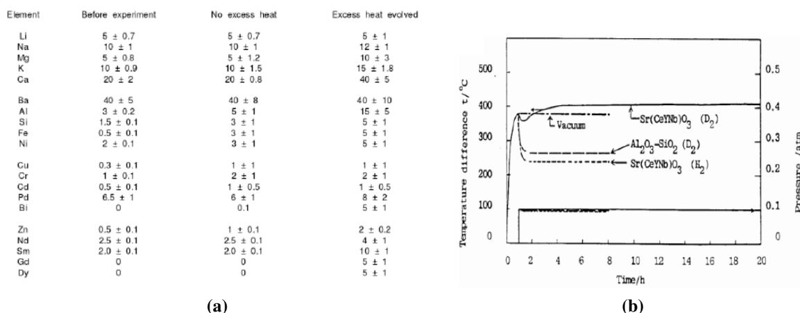
Figure 2. (a) Elemental analysis for impurities in the proton conductor Y-doped \text{SrCeO}_3 , showing the presence increase of several chemical elements after electrolysis. (b) Anomalous heat production during electrolysis. From [6,8].
