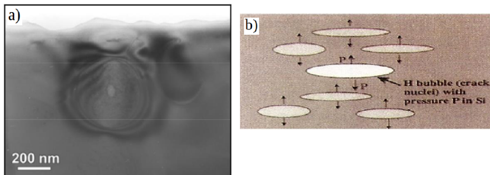
Figure 8. (a) Cross-section TEM image showing a nanometric cavity pressurized by its internal H_2 , and the long-range surrounding strain field, deep under the free surface of a hydrogenated Si wafer below 470 K. From [28]. (b) Diagram showing the pressure of H_2 in nanometric cavities on the Si crystalline matrix. From [29].
