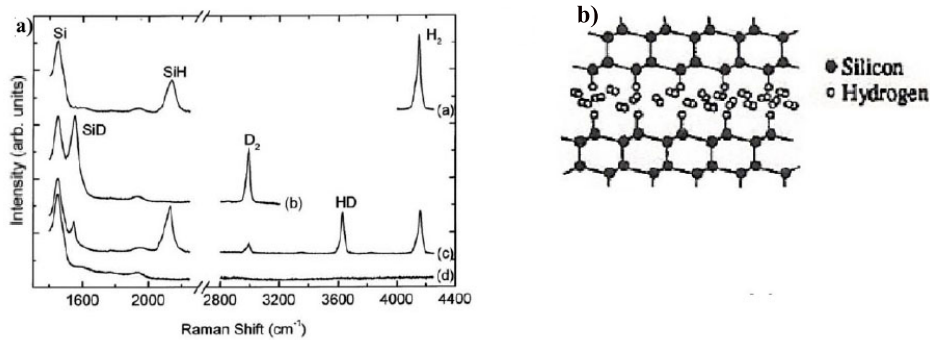
Figure 7. (a) Raman spectroscopy on Si surface implanted with hydrogen ions at 470 K showing the presence of H_2 molecules in nanometric cavities. From [31]. (b) Diagram of H_2 molecules trapped in Si nanometric cavities. From [29].
