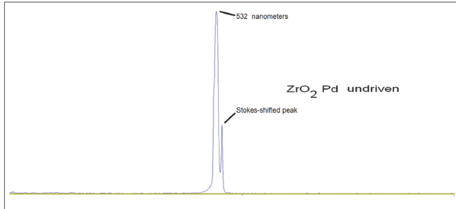
Figure 4. Dual wavelength volume-enhanced reflection spectroscopy of an unloaded, undriven NANOR-type component ( \text{ZrO}_2\text{Pd} ). This material is discussed elsewhere [3,17] and does not give excess heat [7]. Here the CMORE-spectroscopy reveals a clear Stokes peak with small, negligible, anti-Stokes component. This is discussed further below.
