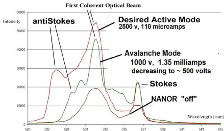
Figure 1. Three different electronic states optical signatures for the same preloaded \text{ZrO}_2\text{PdD} NANOR ® -type CF/LANR component in three different electrical drive modes. Shown are spectra of the same NANOR ® -type CF/LANR component in three different electronic states, resolved by dual wavelength coherent electric-driven volume-enhanced reflection spectroscopy. The three modes (responses) are the undriven “off”-state, the unwanted electrical avalanche mode [7], and the optimal operational state, the “Desired Active Mode”, where “excess” energy is being released.
