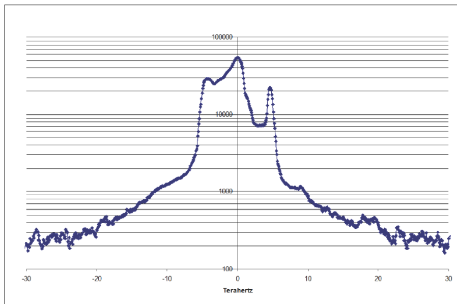
Figure 8. Logarithmic presentation of dual wavelength electric-driven volume-enhanced reflection spectroscopy of a preloaded, correctly driven, \text{ZrO}_2\text{PdD} NANOR ® -type component. The x -axis here presents the frequency difference from the main laser frequency.
