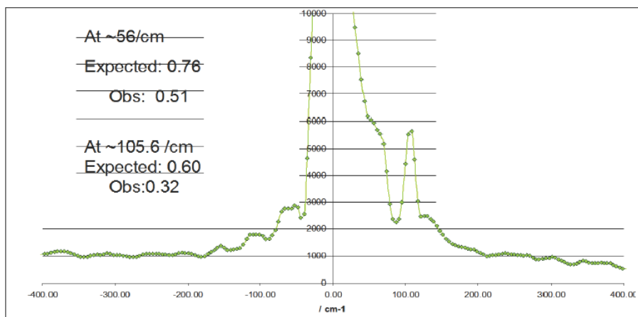
Figure 9. Dual wavelength volume enhanced spectroscopy. The observed optical output of the NANOR ® -type LANR component (containing \text{ZrO}_2\text{PdD} ) with no additional electrical drive/activation, the “off” state, but with an additional static applied magnetic field intensity of approximately 2 T at its peak, abutting the core. The x -axis here is plotted as normally done in Raman spectroscopy with the units of (1/\text{cm}) , to which it is normalized.
