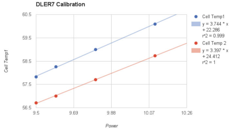
Figure 17. A typical calibration obtained by fitting the steady-state response of the calorimeter to the input power at various steps.
