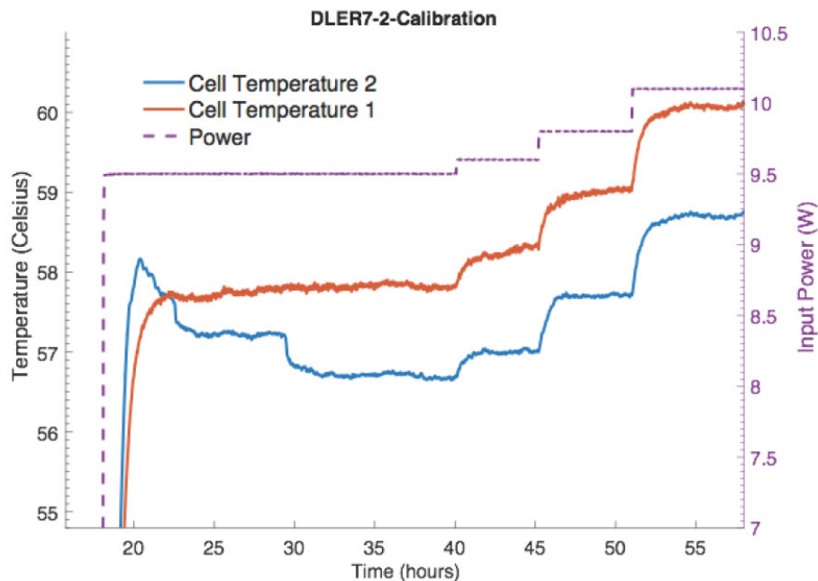
Figure 5. Example of single-thermistor temperature sensing instability.
