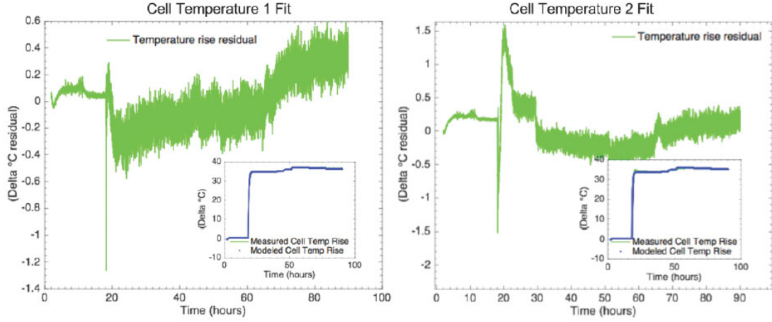
Figure 6. Model fits to the two cell temperature readings obtained during run DLER7-2. Delta (°C) corresponds to temperature difference between cell and enclosure.
