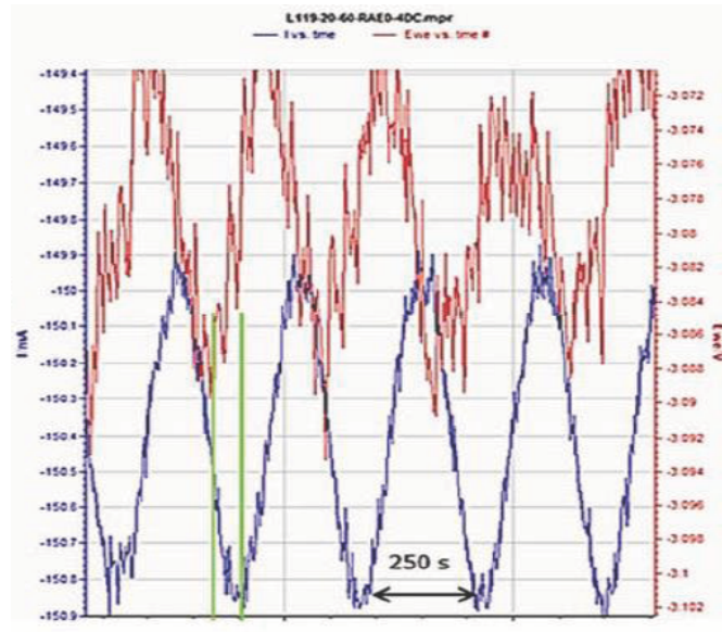
Figure 2. Current ripple at high data acquisition rate.
