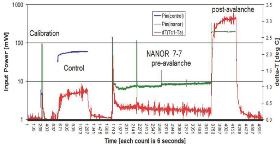
Figure 3. Temperature difference induced by a \text{ZrO}_2\text{-NiD} NANOR ® -type component and ohmic control, both electrically driven, showing both excess heat and avalanche behavior.
