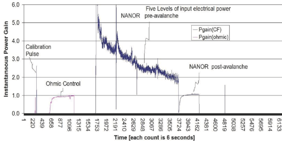
Figure 6. This graph presents the power gain of the \text{ZrO}_2\text{-NiD} NANOR ® -type component CF/LANR component as a function of time, and shows that the excess heat which is generated decreases with high input power, eventually reverting to normal, ordinary, resistor-like operation after the electrical avalanche.
