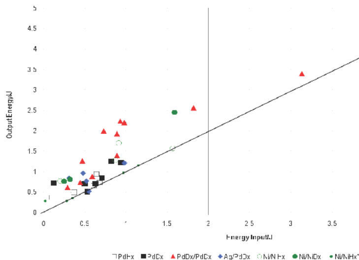
Figure 2. Calorimetrically determined output energy versus Joule input energy for a range of electrochemically loaded wires exercised electrically to destruction.
