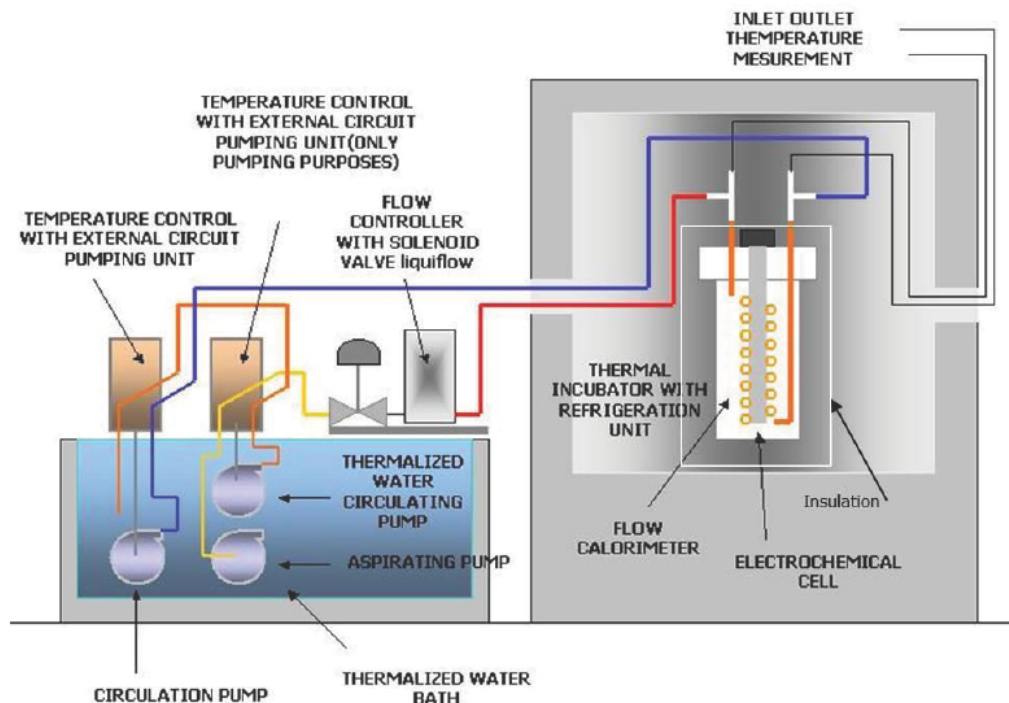
Figure 1. ENEA mass flow calorimeter.
