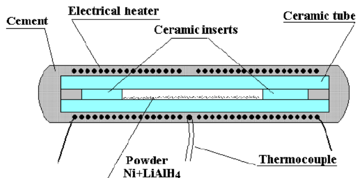
Figure 1. Schematic of the first type device.
