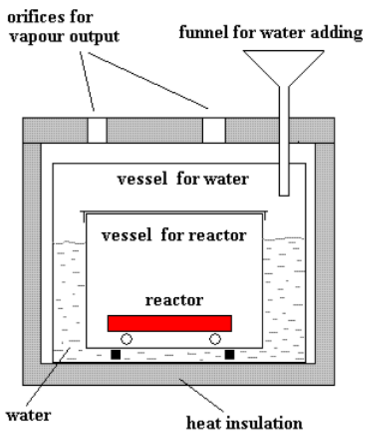
Figure 2. Schematic of the calorimeter with vaporized water.
