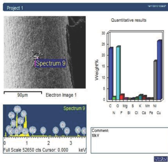
Figure 5. EDX on one of several hot spots detected on the constantan wire. Elements not in the wire composition are: C, N, O, F, Mg, S, K, Cl, and Ca .
