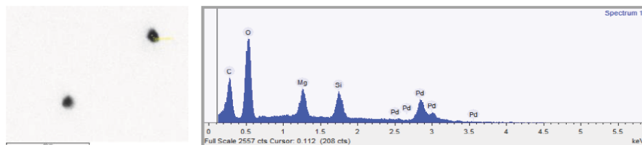
Figure 14. EDX spectrum element list: C, O, Mg, and Si.
