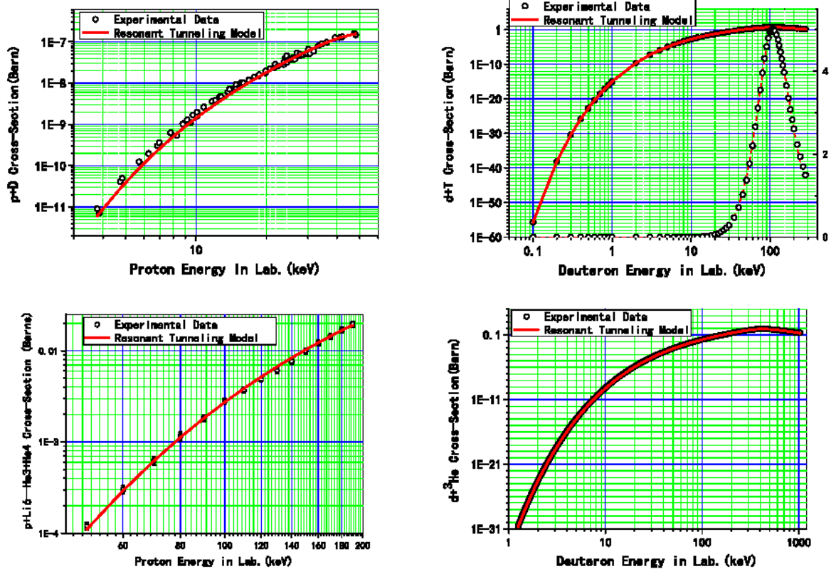
Figure 1. 3-Parameter formula, Eq. (6) is justified by eight sets of fusion cross-section data.
