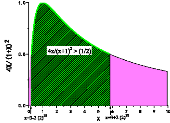
Figure 3. The width of the resonance peak in cross-section is 4(2)^{1/2} .
