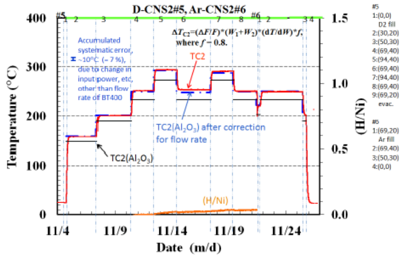
Figure 5. Evolution of the temperature at TC2 in the D-CNS2#5 and Ar-CNS2#6 runs compared with that in the calibration/control run H-Al 2 O 3 3. The corrected reference temperature TC2(Al 2 O 3 ) is calculated by adding \Delta T_{C2} due to deviation of the flow rate of BT400 to the latter.
