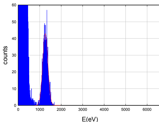
Figure 4. Example of a spectrum from the X-123 detector.
