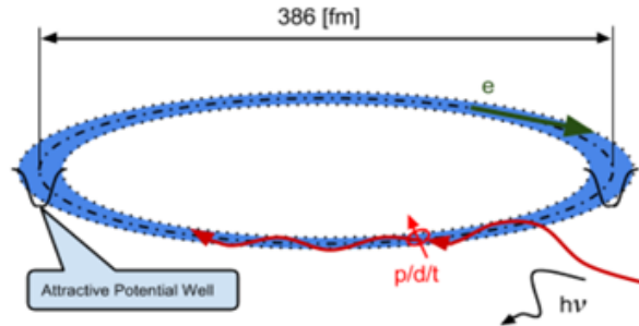
Figure 1. Schemic view of a hydronium with the HNu bound to move along the ZB trajectory.
