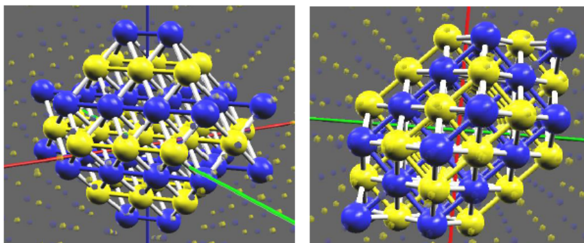
Figure 3. Possible symmetric structure of \text{Ni}^{62} .
