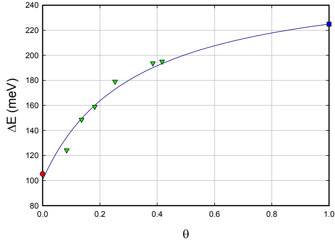
Figure 9. O-site to T-site excitation energy as a function of loading; inferred from data of Pitt and Gray [73] (green triangles); estimated from high pressure loading data of Baranowski et al. [42] (blue square); excitation energy from \alpha -phase PdD x analysis of Hagelstein (2015) (red circle); empirical fit (dark blue line).
