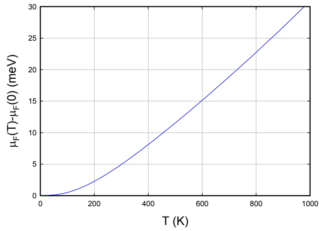
Figure 3. Incremental Fermi level for Pd as a function of temperature.
