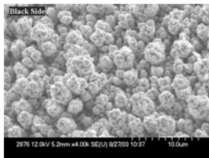
Figure 1. SEM of the Pd/D co-deposited material.
