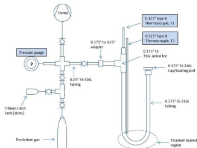
Figure 2. Experimental apparatus for thermal shock experiment.
