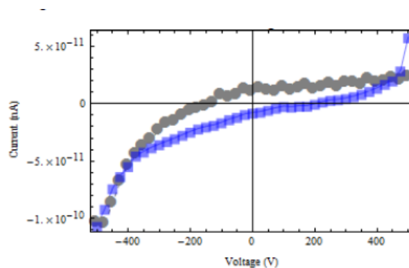
Figure 7. I - V Characteristic of diamond sensor 3 after deuterium loading.
