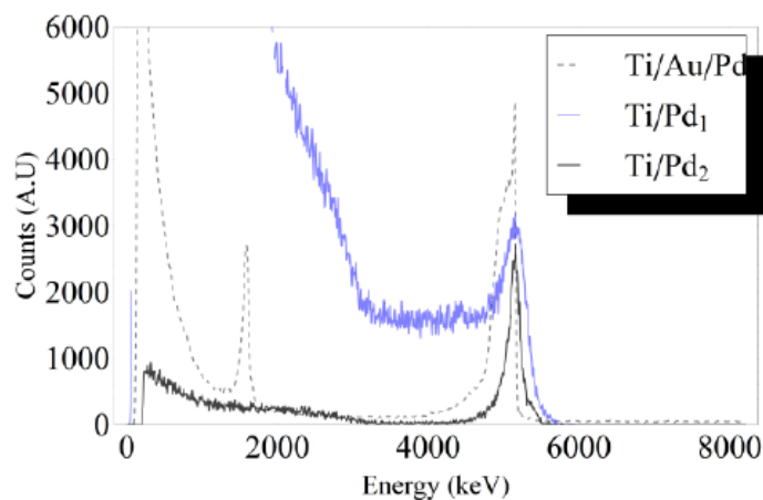
Figure 2. Pu-239 Diamond sensor energy calibration spectra.
