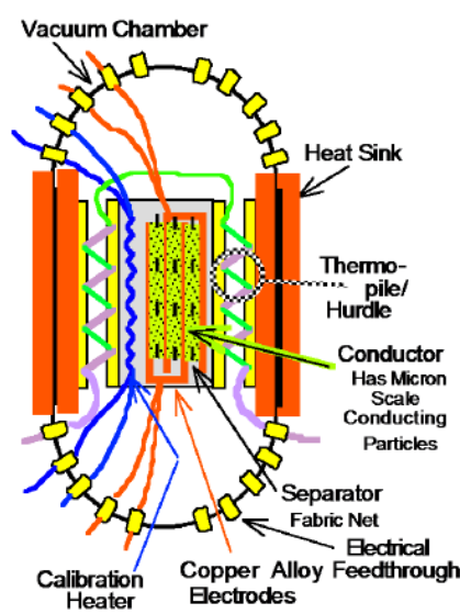
Figure 4. Calorimeter assembly.
