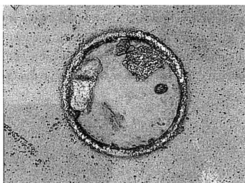
Figure 35. Ring track of Matsumoto
