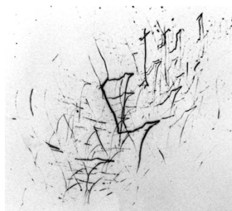
Figure 24. Vector Swarm Group correlation of tracks including random motion components. These tracks do not line up when overlaid. They change form with location, apparently due to relative position in the applied non-uniform magnetic field. A large number of the tracks in this exposure are correlated. A measure of corresponding line segments of matching groups of tracks reveals a macroscopic “central force,” which will be the subject of future work.
