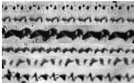
Figure 11. Different types of positive regular periodic structure tracks in Polychrome Litho film, no pre-exposure, developed with constant agitation.
