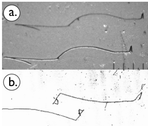
Figure 2. (a) Fredericks tracks. Correlated tracks in Kodak Kodalith type III film. Tracks are copies instead of mirror images or chirally transformed. (b) Ivoilov “chiral” tracks. Multiple correlated tracks can be seen in the original image. The chirally transformed track is explained in the Ivoilov analysis as a reflected track which is recorded on the bottom emulsion facing an aluminum plate with polyester base material sandwiched between the two emulsion layers. Unspecified type of double-sided X-ray emulsion.
