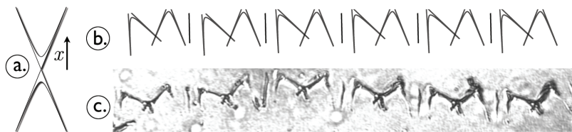
Figure 36. (a) Intersection of tachyon with plane parallel to particle motion on x axis. (b) Simulation of “M” components of track with periodic structure using conic sections. (c) Track from Fig. 4 exhibiting periodic structure.
