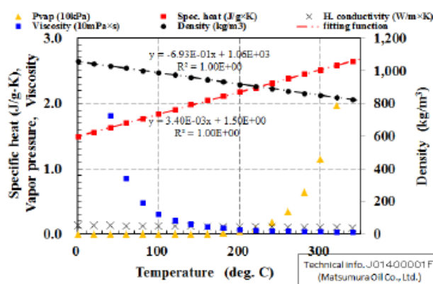
Figure 2. Physical properties of BarrelTherm-400.
