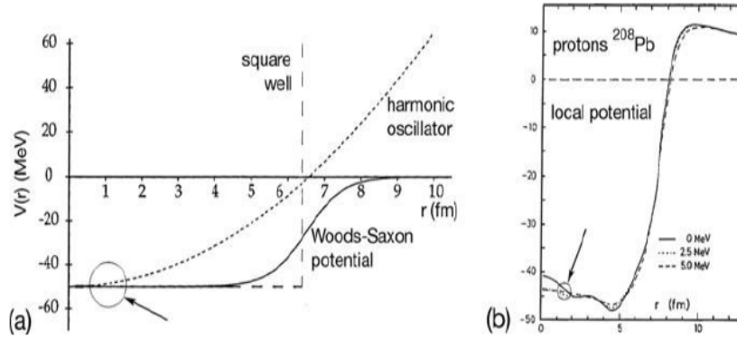
Figure 3. (a) A nuclear-potential model and two simplifying approximations. (b) A measured nuclear-potential profile.
